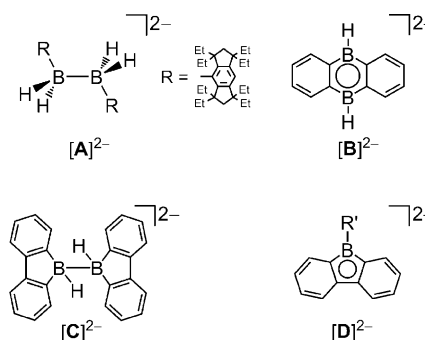
Figure 1. The isolable [H_3B–BH_3]^{2-} derivative [A]^{2-} , the \pi -delocalized 9,10-diborataanthracene [B]^{2-} , and their 9-borafluorene analogues [C]^{2-} and [D]^{2-} , respectively.
